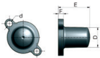
Protective cap SK
